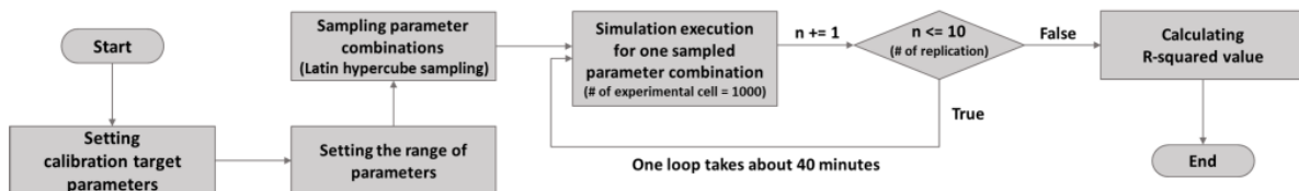
Figure 8: Flow chart of output validation process
