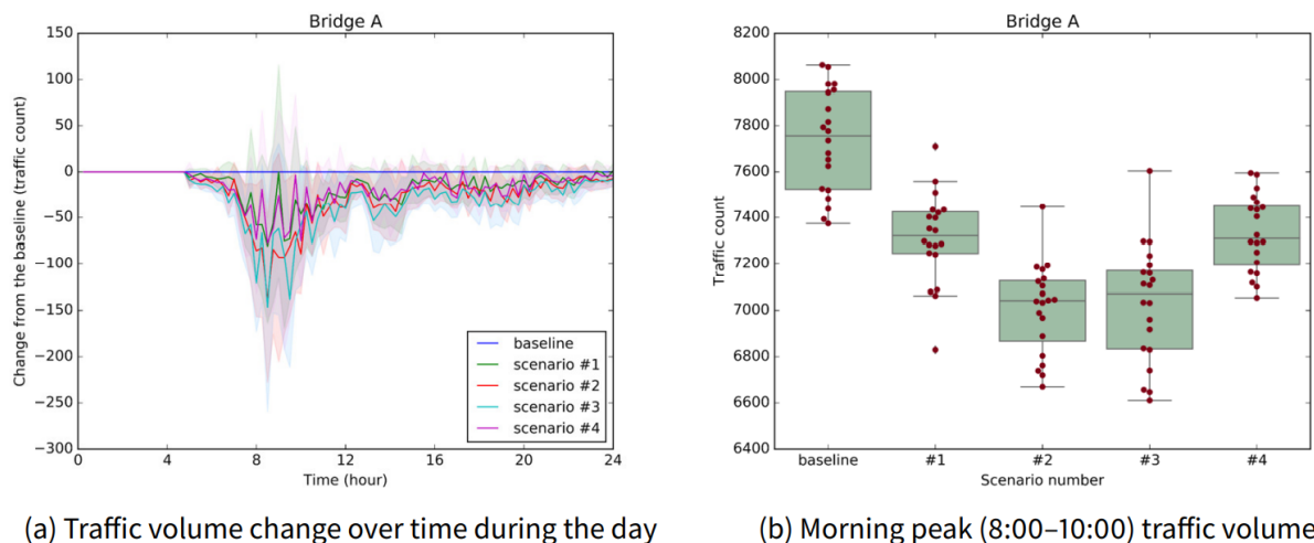
Figure 10: Traffic volume comparison by new bridge construction scenario ( Bridge A )
